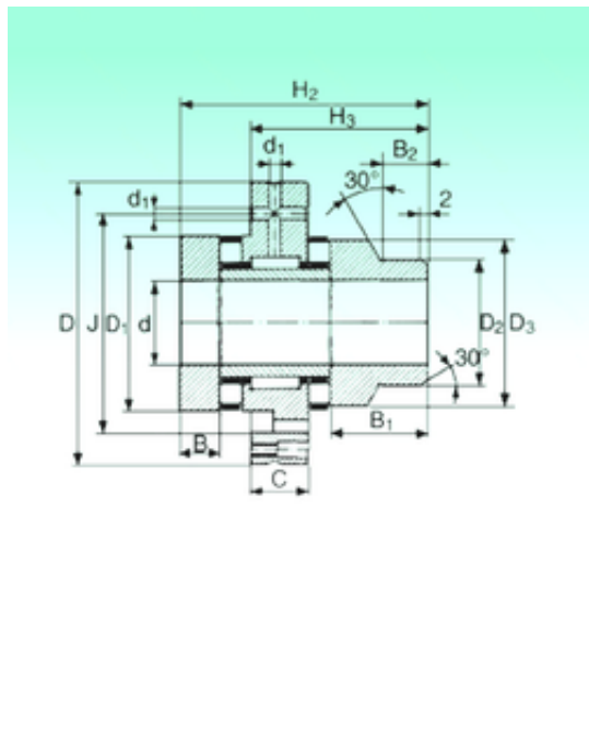
ZARF 30105 L TN Bearing 2D drawings and 3D CAD models
