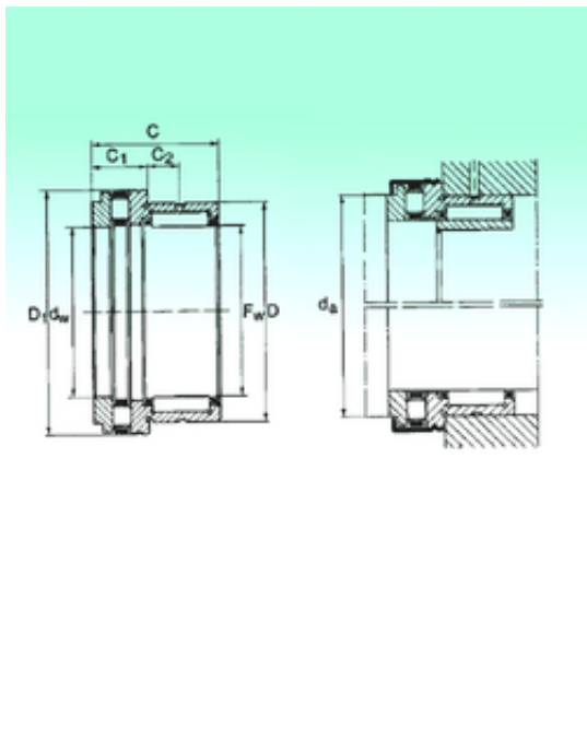
NKXR 45 Bearing 2D drawings and 3D CAD models
