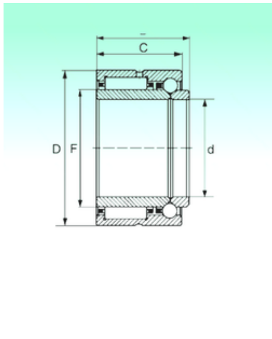
NKIB 5911 Bearing 2D drawings and 3D CAD models
